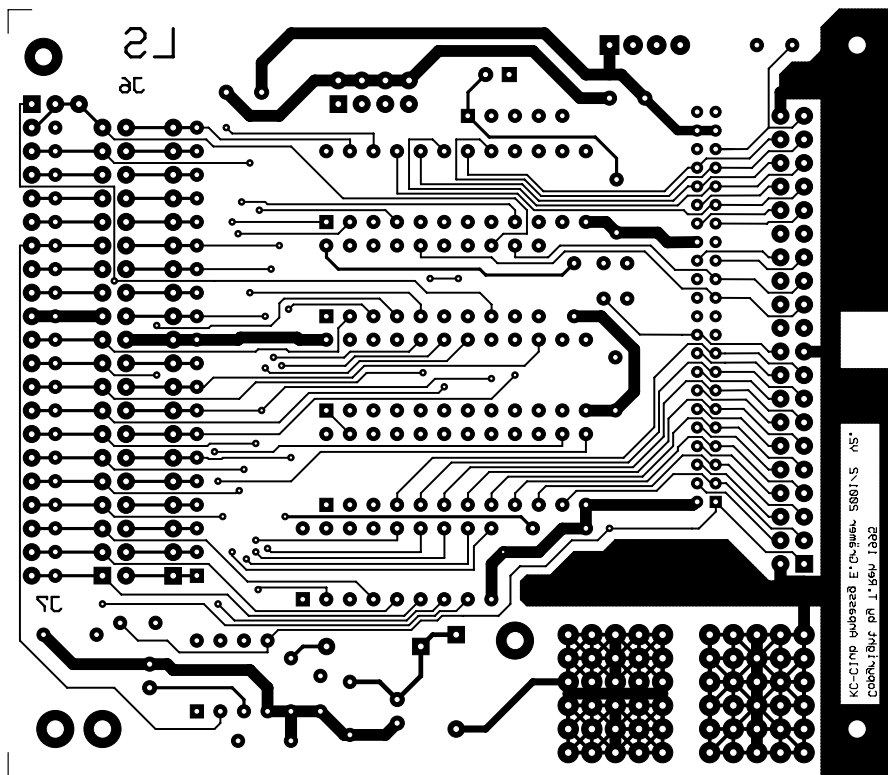
Figure 3: PCB layout, solder side
