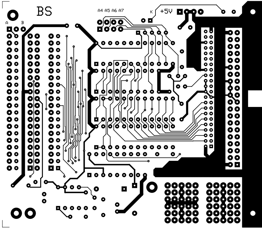
Figure 2: PCB layout, component side
